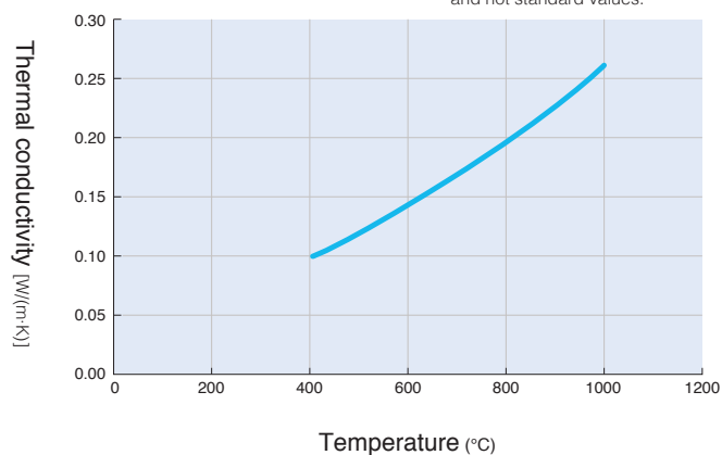
Thermal conductivity of TOMBO No.5625-A/M
