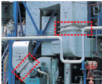
BELLOW-Q™ (non-metallic flexible expansion joints)
