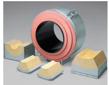
FOAMNERT™ Support (Rigid urethane supports)
