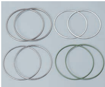
Metal O-Seal™ Hollow metal O-ring for a wide variety of applications
