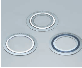
VORTEX™ gasket (spiral wound gasket) Metallic gasket that are ideal for conditions ranging from extreme low temperatures to high temperatures
